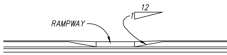
CURB RAMP DETAIL 2
