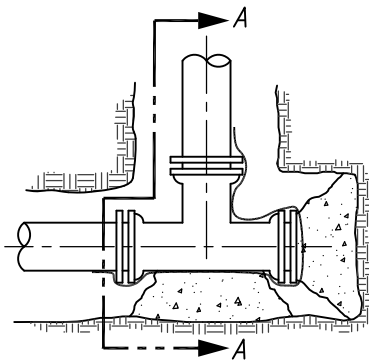
TEE W/ DEAD END BRANCH
