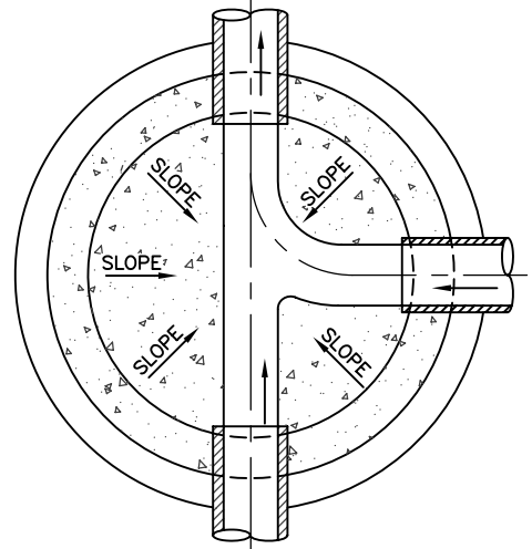
"J" JUNCTION
