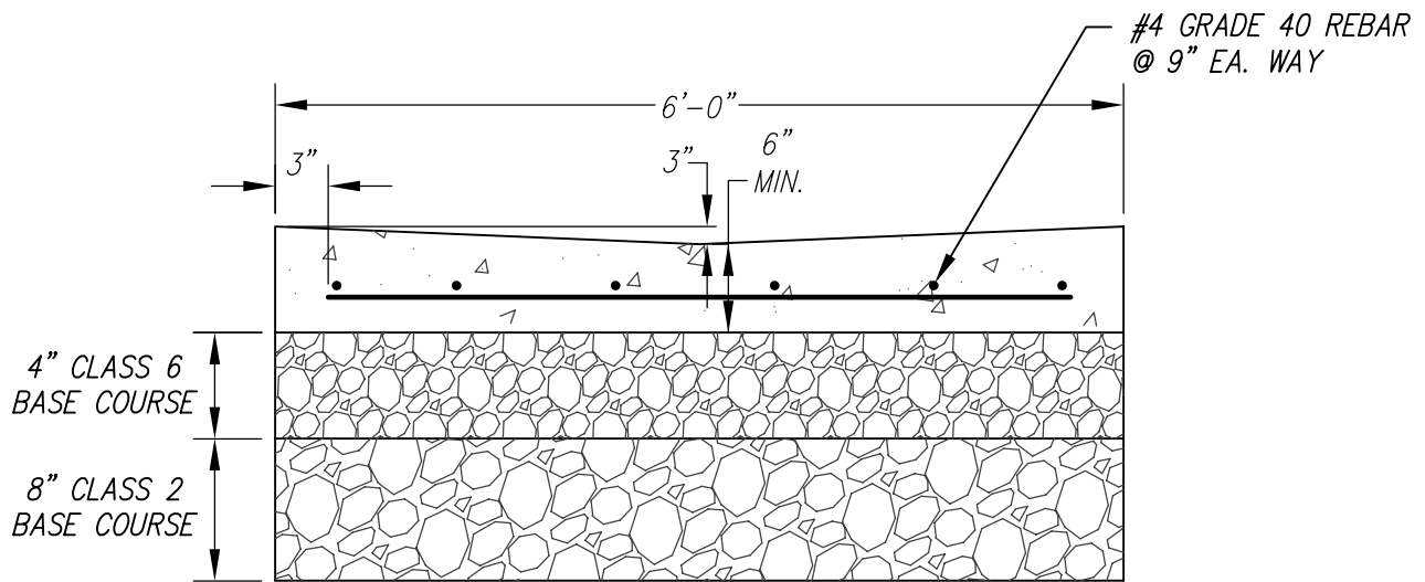
VALLEY GUTTER SECTION
