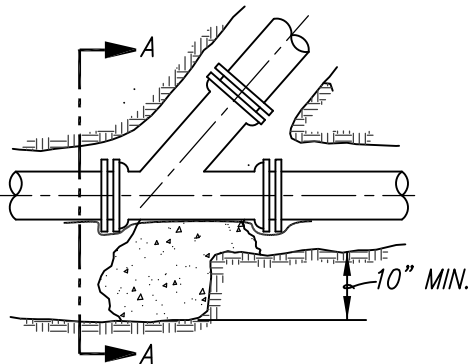
WYE
